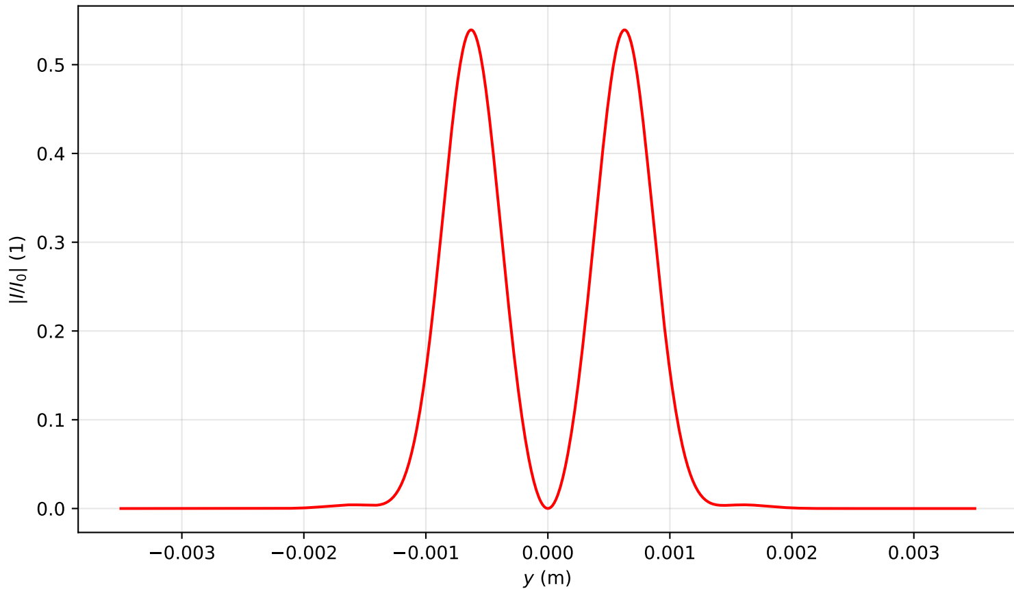
Intensity profile I(x=0, y, z=1.353)/I_0 , \text{Pin}=3.0\text{Pcr} , artificial time
